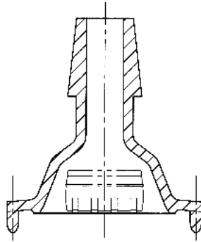
Figure 2, NPP-301 Pressure Connection
