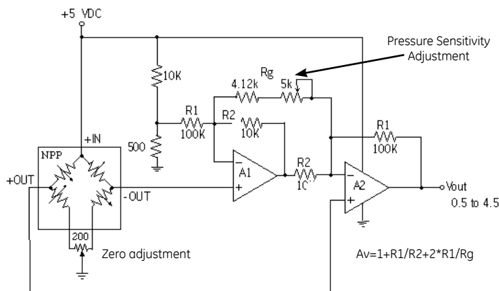
Figure 3. Amplifier Circuit for NPP-301
