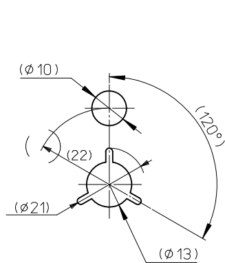
DETAIL "F"
