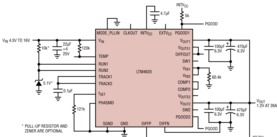
26A, 1.2V Output DC/DC \mu Module ® Regulator
