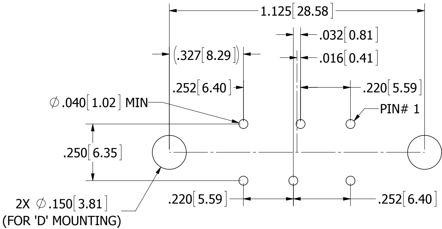
PCB LAYOUT RECOMMENDED (COMPONENT SIDE)
