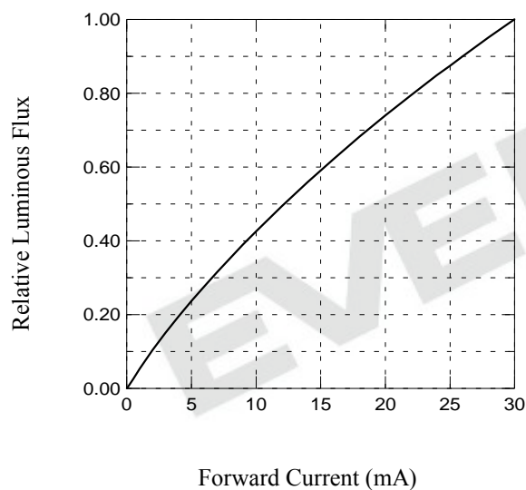
Relative Luminous Flux vs. Forward Current ( T_a=25^\circ\text{C} )
