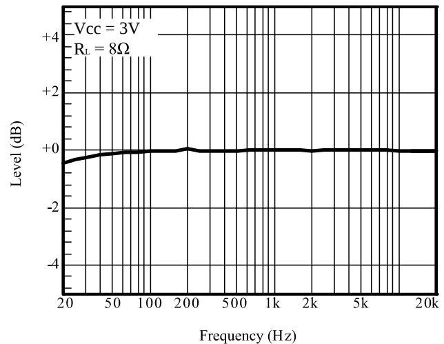
Figure 13 Frequency Response
