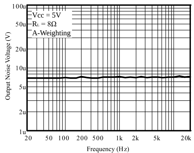
Figure 11 Noise Floor
