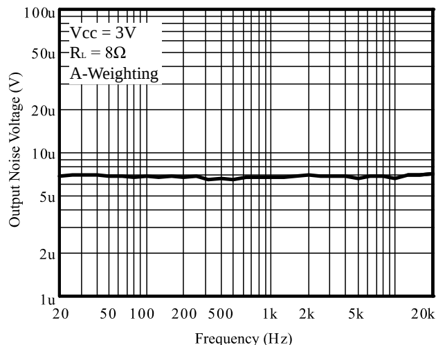
Figure 15 Noise Floor
