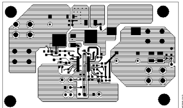
Figure 14. Top Layer
