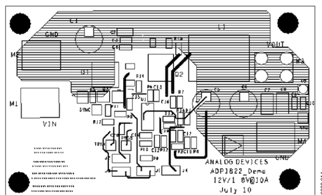
Figure 15. Bottom Layer
