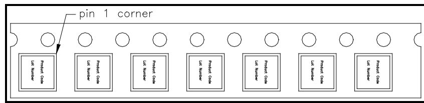
Figure 7: SE2604L-R Tape and Reel Information
