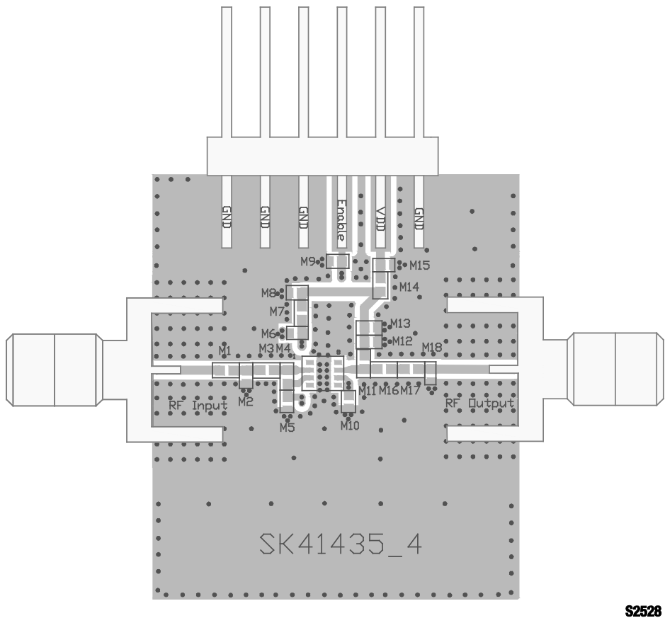
Figure 26. SKY67003-396LF Evaluation Board Assembly Diagram
