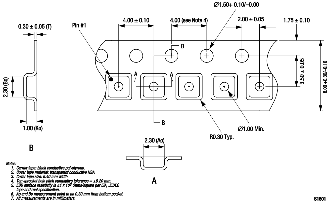
Figure 32. SKY67003-396LF Tape and Reel Dimensions
