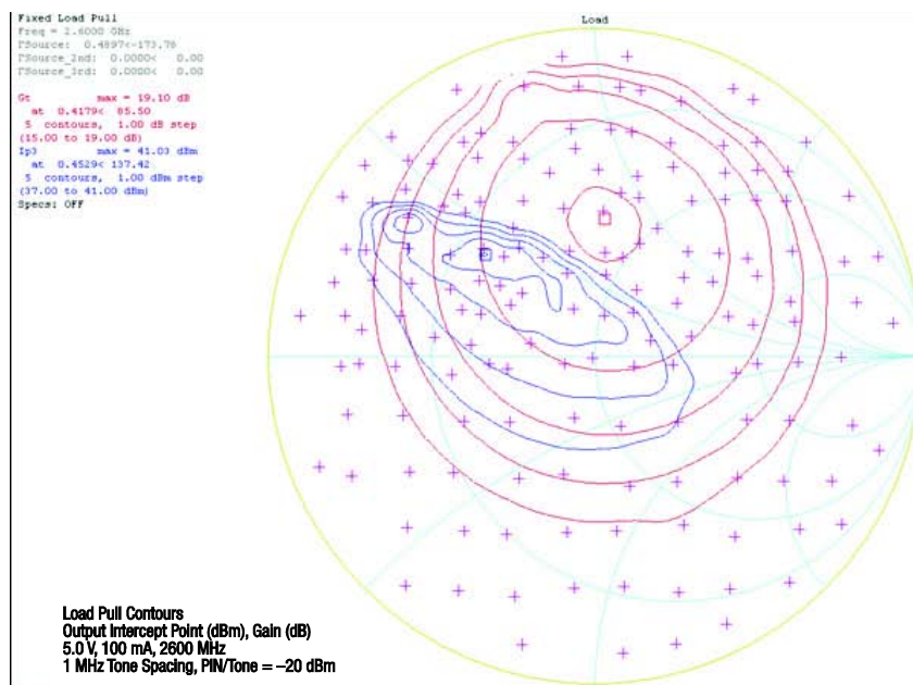
Figure 25. Load Pull, @ 5 V, 2600 MHz, 100 mA
