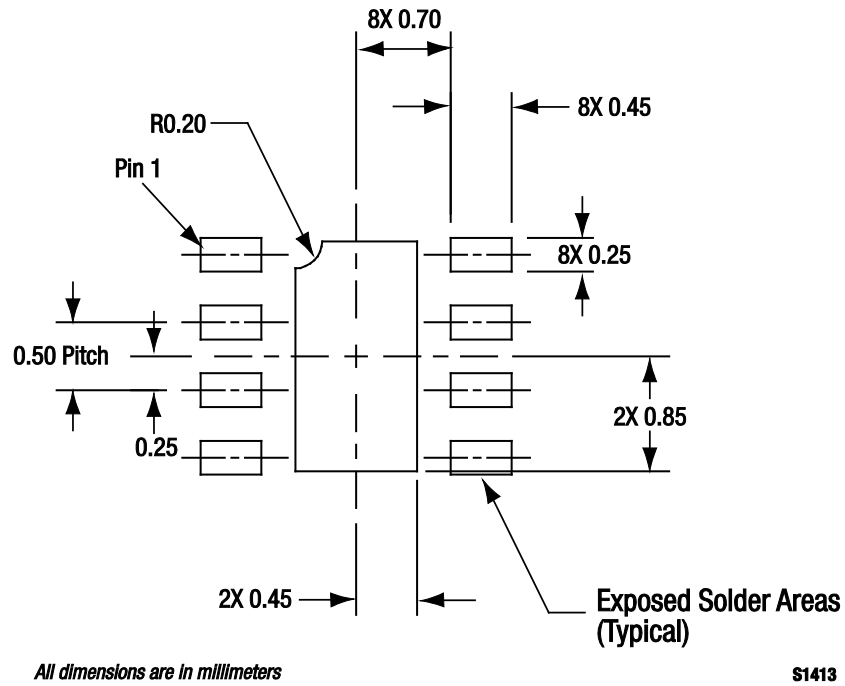
Figure 29. SKY67003-396LF PCB Layout Footprint (Top View)
