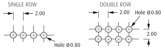
Recommended PC Board Patterns
