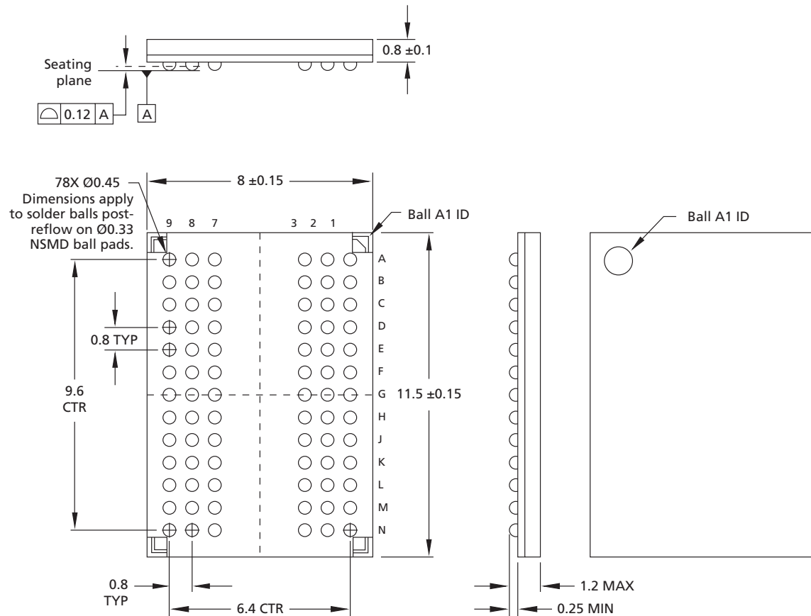
Figure 8: 78-Ball FBGA – x4, x8 (JP)
