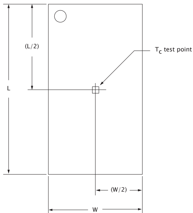
Figure 10: Thermal Measurement Point
