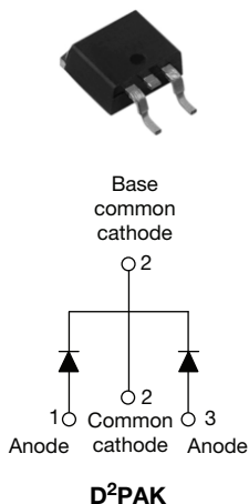
VS-15CTQ...SPbF
