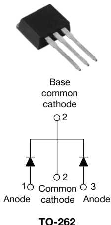
VS-15CTQ...-1PbF
