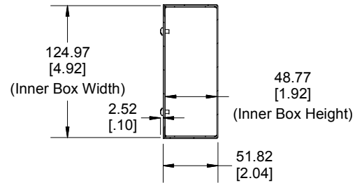
SECTION A-A End View of Assembly
