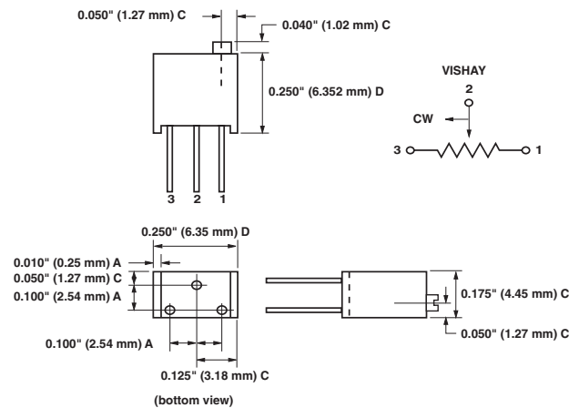
FIGURE 1 - SCHEMATIC AND DIMENSIONS in inches (millimeters)
