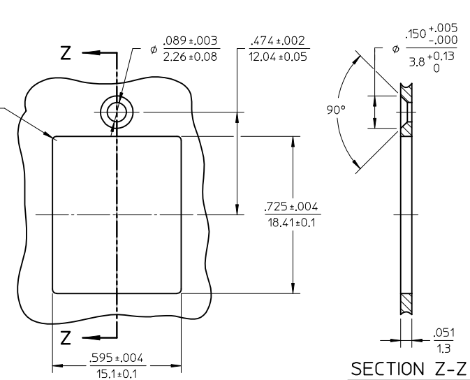
RECOMMENDED MOUNTING PATTERN SCALE 2.5:1
