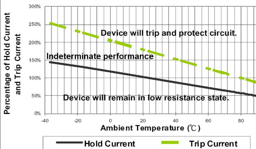
Hold & Trip Current and Thermal Derating Curve
