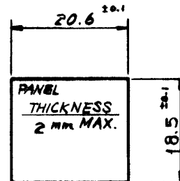
MOUNTING HOLE DETAIL (SCALE 1:1)
