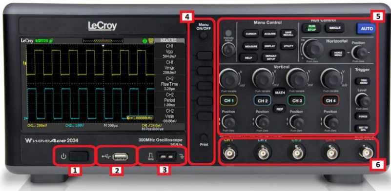
Front panel buttons and knob locations on 4 Channel WaveAce Oscilloscopes. Layout is very similar on 2 Channel models
