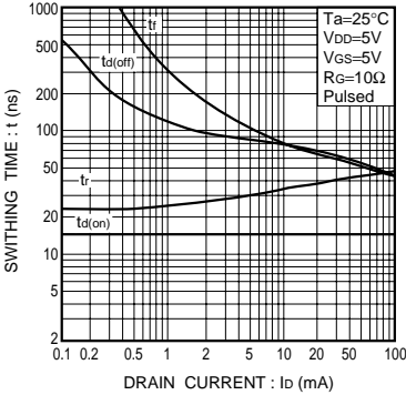
Fig.19 Switching characteristics
