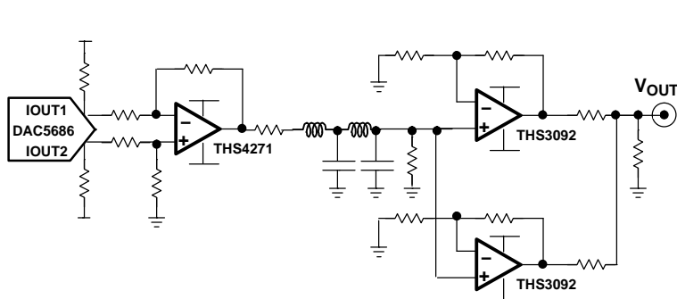
TYPICAL ARBITRARY WAVEFORM GENERATOR OUTPUT DRIVE CIRCUIT
