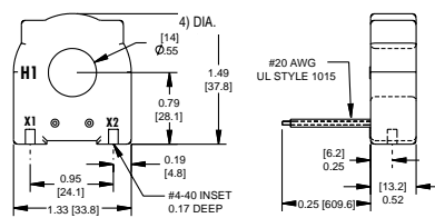
Model 18 Dimensions
