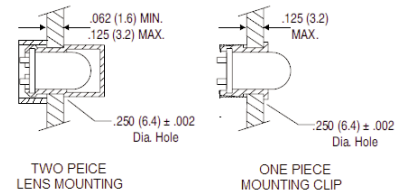
PH25 Mounting
