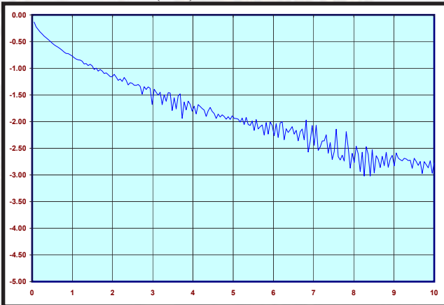
PN: CCSMA-MM-SS402-60 INSERTION LOSS (S21)
