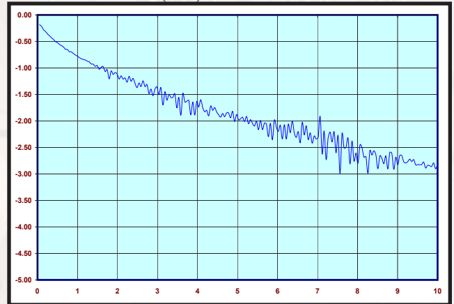
PN: CCSMA-MM-SS402-60 INSERTION LOSS (S12)
