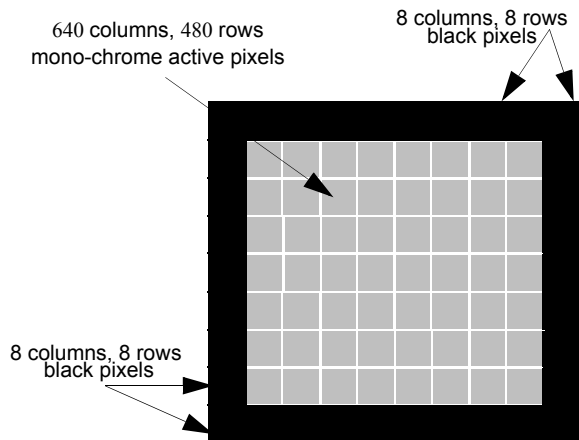
Figure 7: CMOS APS region of the LM9619
