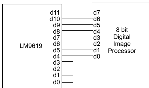
b) LM9619 Connected to a 8 bit Digital Image Processors
