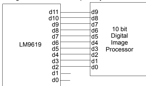
a) LM9619 Connected to a 10 bit Digital Image Processors
