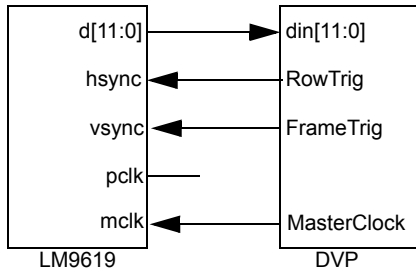
Figure 48. LM9619 in slave mode
