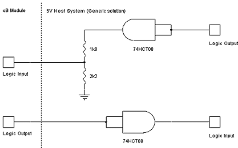
Figure 13: Interface example with logic levels to a 5V system. The gate converting from host 5V output to module input can be replaced with an LVC gate if the voltage divider is removed.
