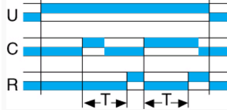
Function Ad - 1 relay output
